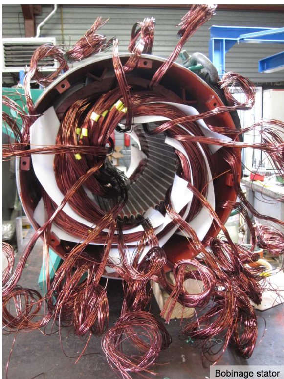
Bobinage stator
